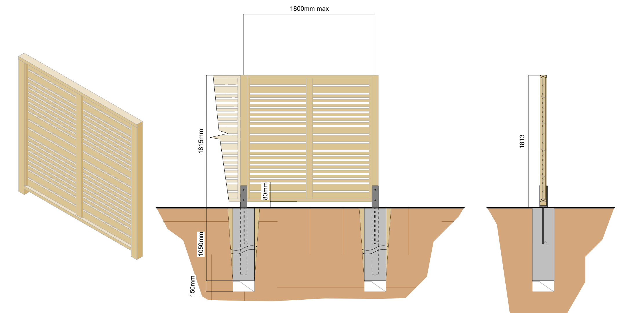
1 1.8m Ht Wood Privacy fence with 4x4 post Scale: 1:30
